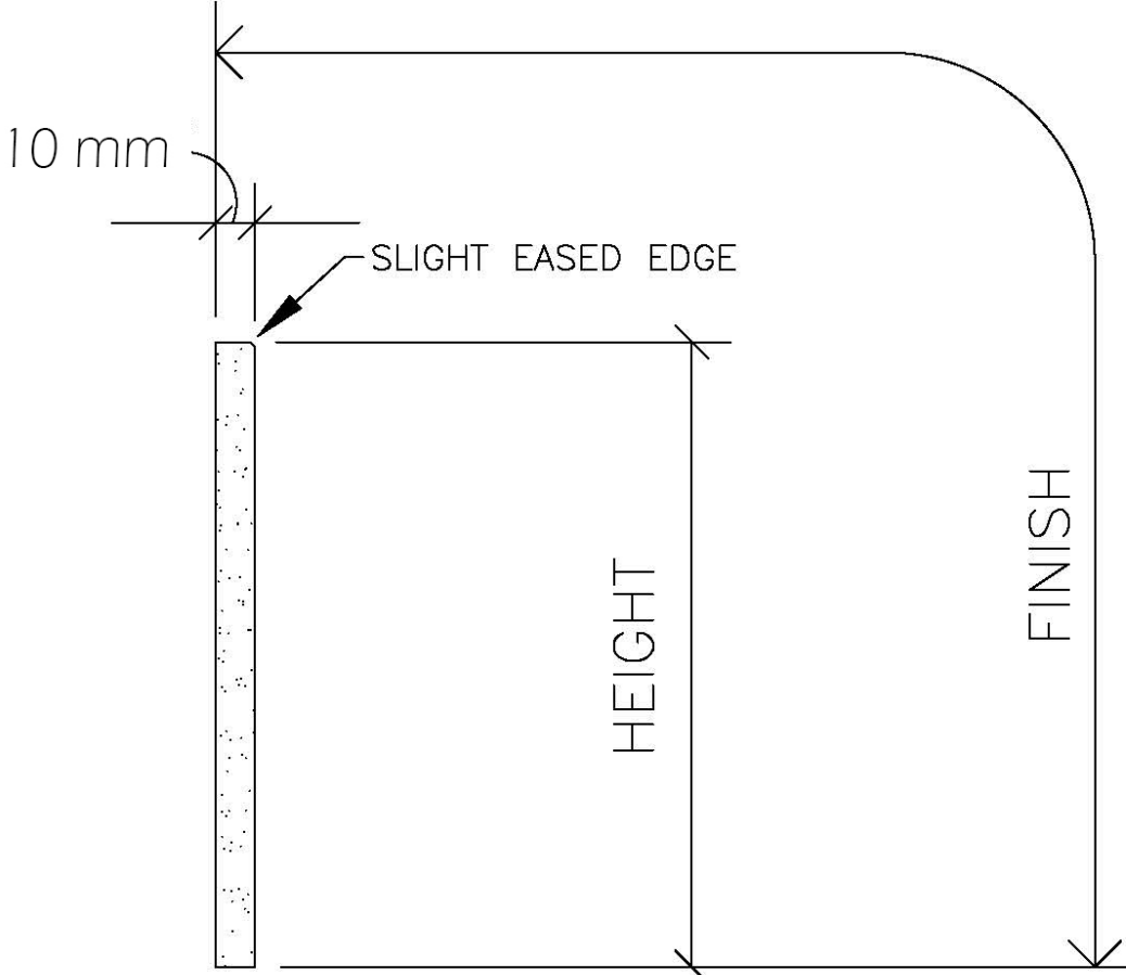
STRAIGHT BASE SECTION
