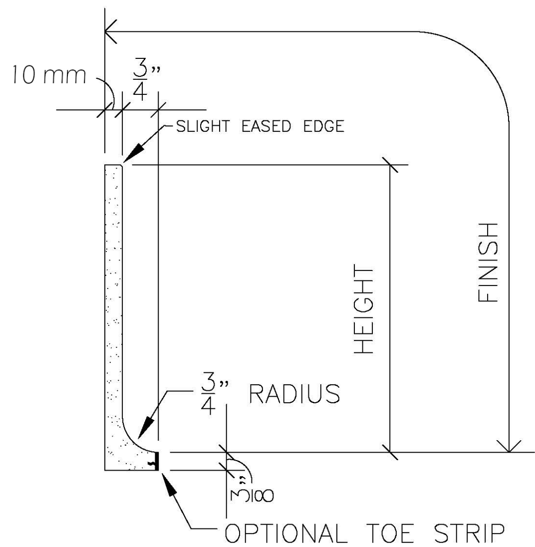
COVE BASE SECTION
